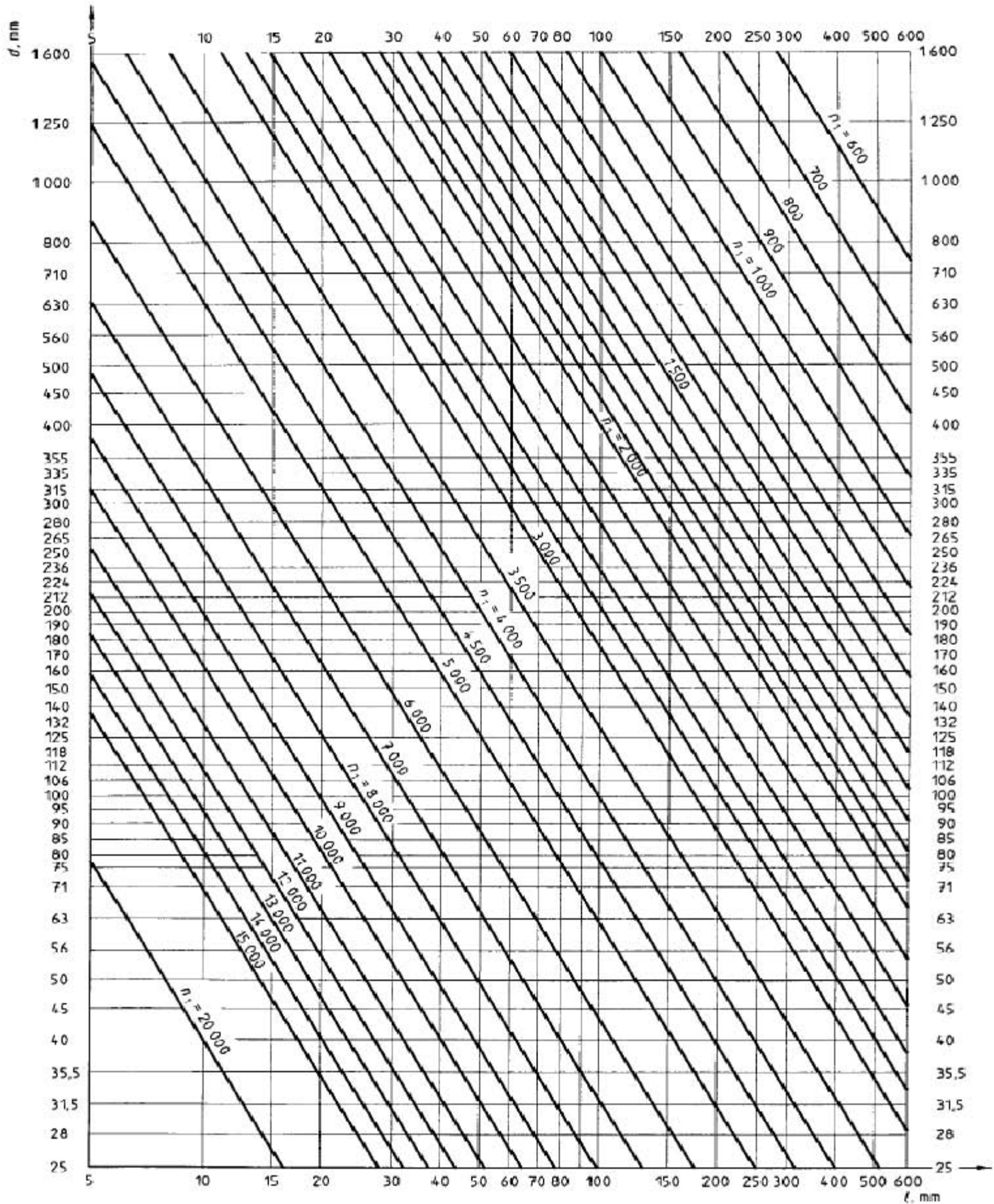
Figure 1 — Limit n_1 ( \text{min}^{-1} ) for static or dynamic balancing
